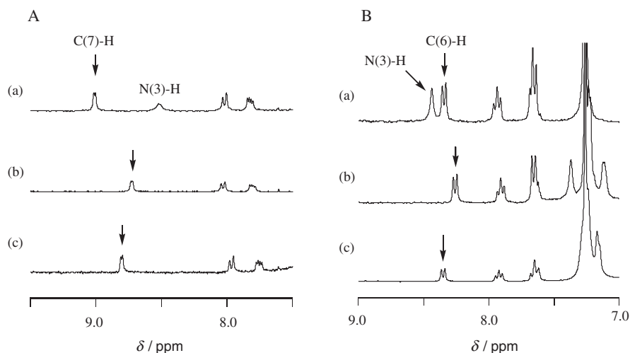
Fig. 4. ^1\text{H} NMR Spectra of 6-AzaFl (A) and Fl (B). (a) Flavin, (b) Flavin + 1 , (c) Flavin + 2 . [flavin] = [ 1 ] = 2.5 \times 10^{-3} M, [ 2 ] = 5.0 \times 10^{-3} M, \text{CDCl}_3 , 25^\circ\text{C} .
