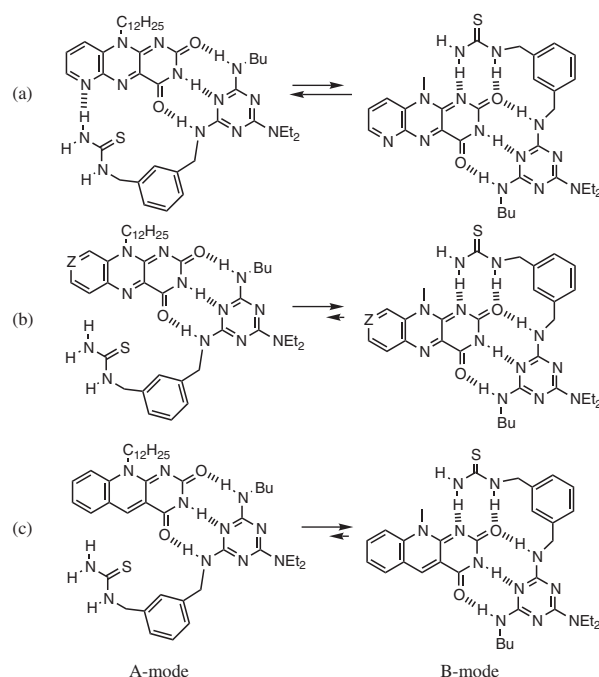
Fig. 3. Possible complex structures of the flavin mimics with 2 .
