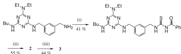
Scheme 1. Synthetic routes of 2 and 3 . (i) PhCOCl, NH 4 SCN, acetone, reflux, 3 h, (ii) 10% NaOH, 90 °C, 4 h, (iii) MeI, MeOH, r.t., 13 h.
