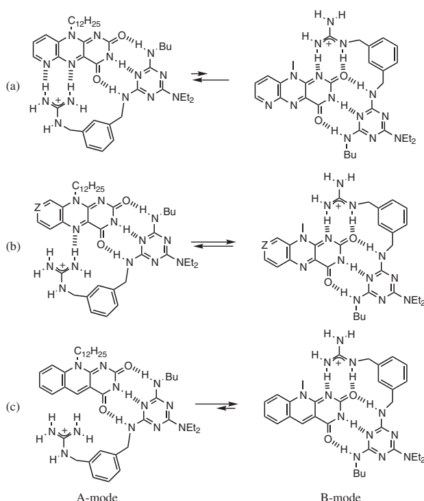
Fig. 2. Possible complex structures of the flavin mimics with 1 .
