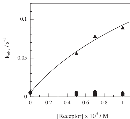
Fig. 7. Concentration effects of receptors on the rate of the oxidation of PhSH: [8\text{-AzaFl}] = 5.0 \times 10^{-5} \text{ M} , [\text{PhSH}] = 5.0 \times 10^{-3} \text{ M} , [\text{Bu}_3\text{N}] = 1.0 \times 10^{-2} \text{ M} , \text{CHCl}_3\text{:MeCN} = 4\text{:1} , \text{N}_2 , 25^\circ\text{C} . \blacktriangle ; 1 , \bullet ; 2 , \blacksquare ; 3 .
