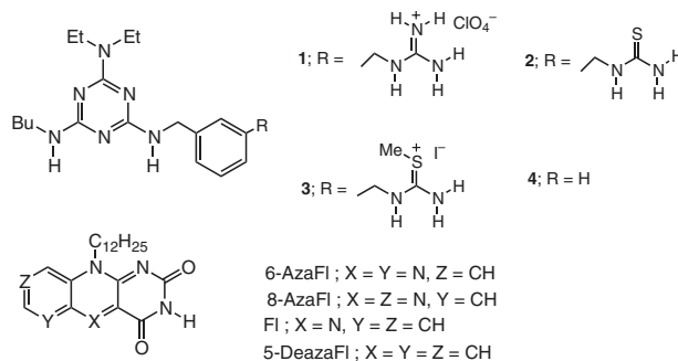
Chart 1. Receptors and flavin mimics.
