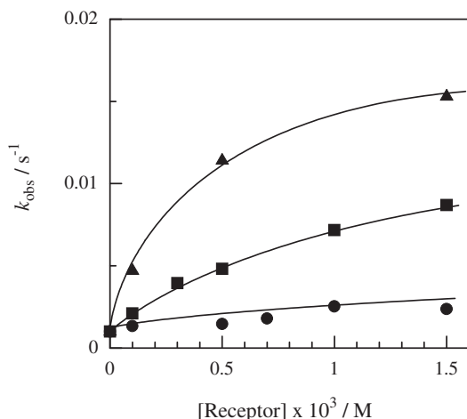
Fig. 6. Concentration effects of receptors on the rate of the oxidation of BNAH: [8\text{-AzaFl}] = 5.0 \times 10^{-5} \text{ M} , [\text{BNAH}] = 4.0 \times 10^{-3} \text{ M} , \text{CHCl}_3 , \text{N}_2 , 25^\circ\text{C} . \blacktriangle ; 1 , \bullet ; 2 , \blacksquare ; 3 .
