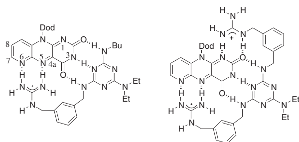
Fig. 1. Complex structures of 6-AzaFI and melamine derivatives bearing guanidinium ion(s).
